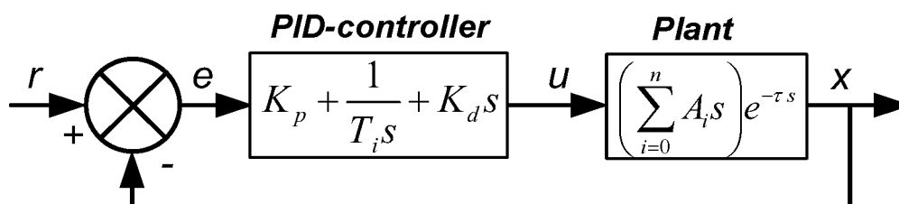
Figure 1. Scheme of the closed-loop controlled plant
