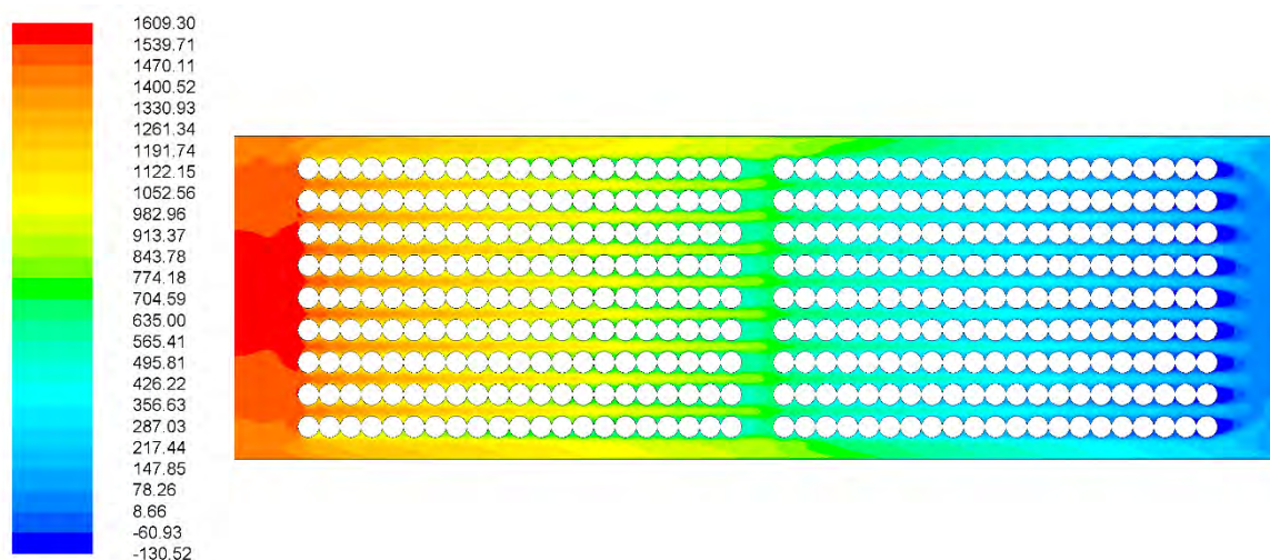
Contours of Total Pressure (pascal)
