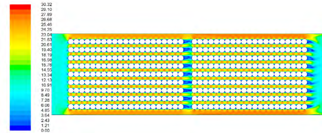
Contours of Velocity Magnitude (m/s)
