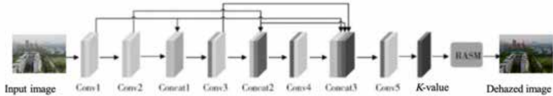
Fig. 2. AOD-Net Network Structure Diagram
