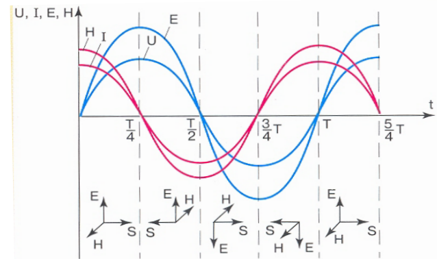
Fig. 6. Direction of the Poynting vector \vec{S} along the single-conductor line in the standing-wave regime: I, H – waves of the current and the magnetic field strength; V, E – waves of the voltage and the electric field strength.
